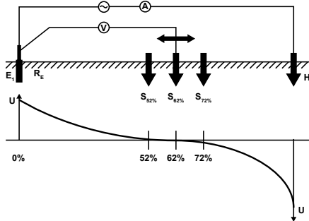
Distribution of voltage during the flow of the test current
